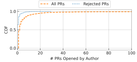
Figure 8: Pull Request Acceptance: The x-axis corresponds to the total and rejected number of pull requests opened by individual authors. Over 60% of authors have no rejected pull requests.
