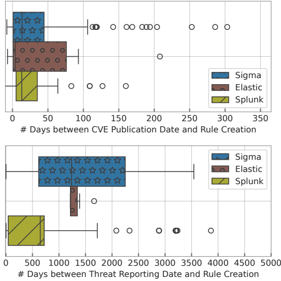
Figure 3: Comparing Reactivity to CVEs and Other Threats: All three repositories have a median reaction time within 2 weeks of a CVE’s publication. The reactivity to attack campaigns and threat groups in the bottom subplot is much larger due to threat disclosures occurring years before the repository creation.
