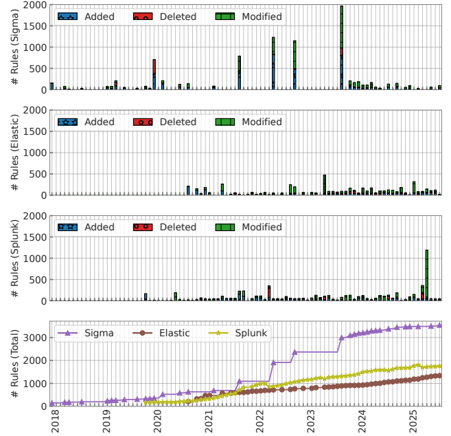
Figure 2: Longitudinal Rule Modification Activity: The y-axis of the top 3 subplots indicates the number of rule queries that have been added, deleted, or modified between tagged releases. Only modifications to the detection query are reported (not the rule metadata). If there was more than one tagged release in a month, the deltas are aggregated. The bottom subplot shows the progression of total number of rules per ruleset, with markers indicating months with an official release (e.g., Sigma had two official releases in 2022).
