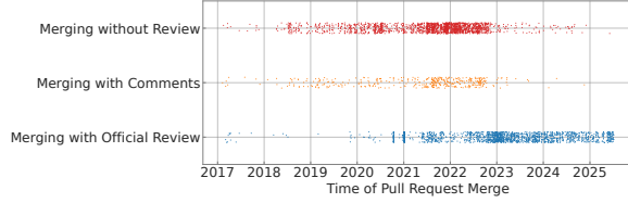
Figure 10: PRs Through the Years: Pull requests are either merged without review or comments, merged with only comments, or merged through the official GitHub review mechanism. The x-axis shows the occurrence of each category of pull requests over time. As the repository has grown, the maintainers have more predominantly used the official mechanism for pull request reviews.
