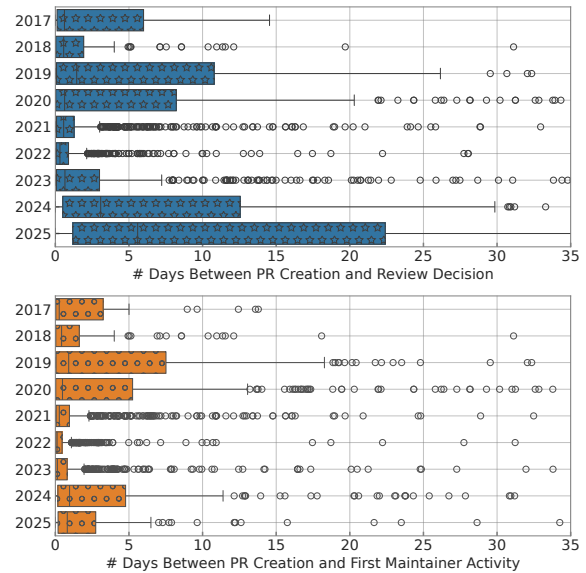
Figure 9: Time to Pull Request Review: Maintainers have consistently responded to new pull requests within a day over the course of the repository history.
