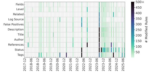
Figure 4: Modifications to Metadata: The y-axis is sorted by total modifications, with the most frequently modified field being Tags . We exclude fields that do not provide context or interpretive value when deploying rules (e.g., Date ; changes to this field are largely specification related).
