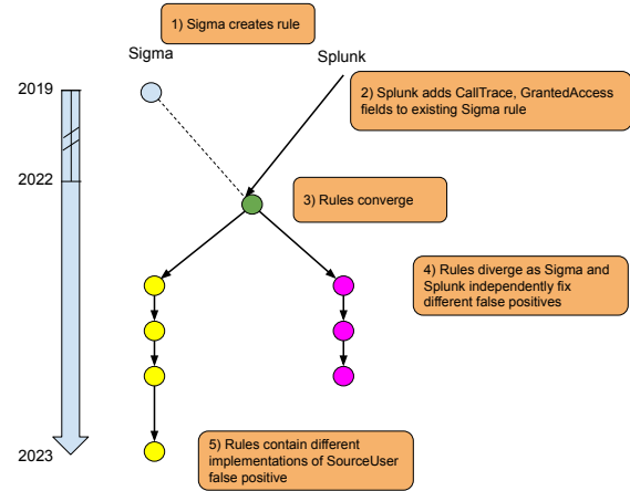
Figure 11: Convergence and Divergence of a Credential Dumping Rule: These rules from Sigma and Splunk converge in 2022 due to a contribution from a Splunk developer to Sigma. Since then, the two repositories have independently made edits to their versions of the rules, causing divergence.
