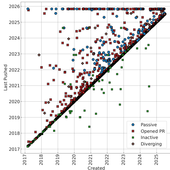
Figure 7: Fork Activity: We compare the fork creation time (x-axis) with the time of the last pushed commit (y-axis). Despite the majority of forks being inactive, there is a broader network of Sigma users that passively ingest rules and make their own changes.
